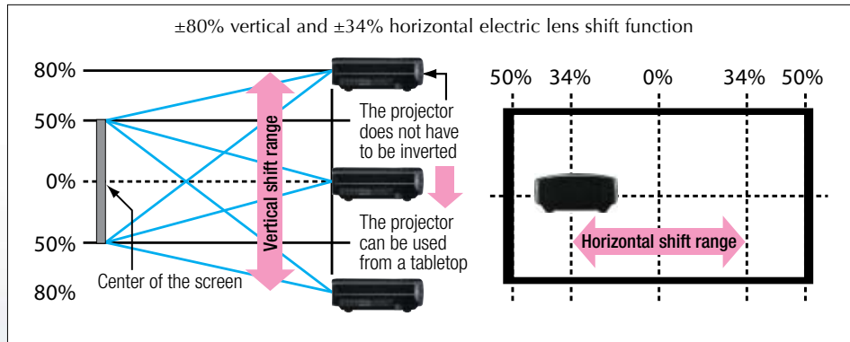
The vertical and horizontal lens shift function cannot be set to the maximum values simultaneously.
